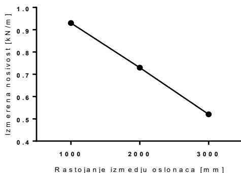
Tip PNK 500/50
