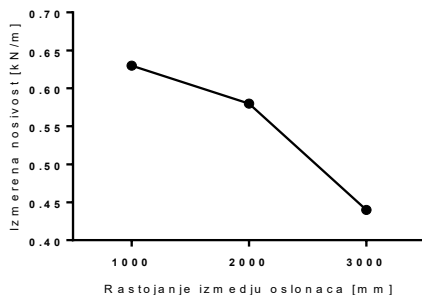
Tip PNK 50/50
