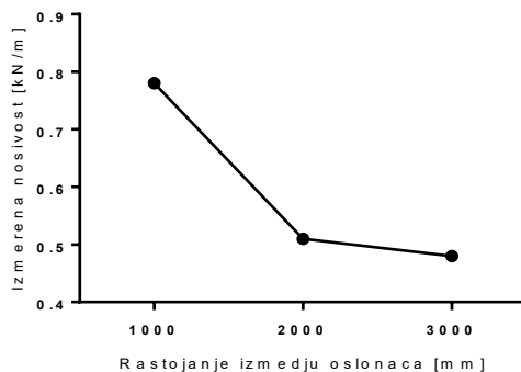
Tip PNK 160/50
