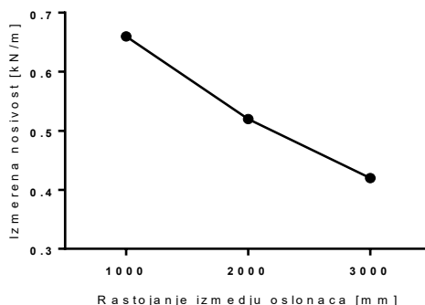
Tip PNK 100/50
