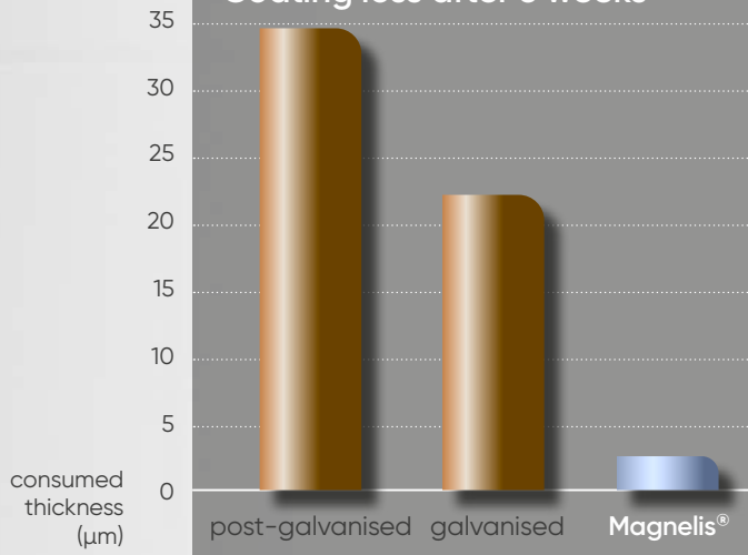
Coating loss after 6 weeks
